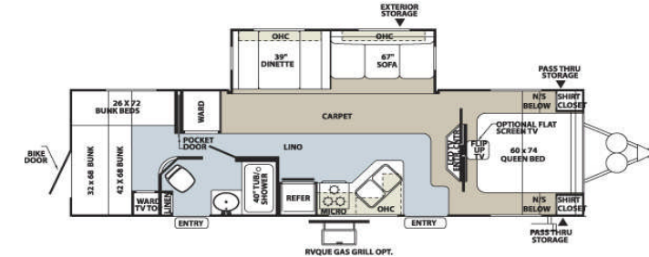
831DBSS 34'1" - 10,39m
