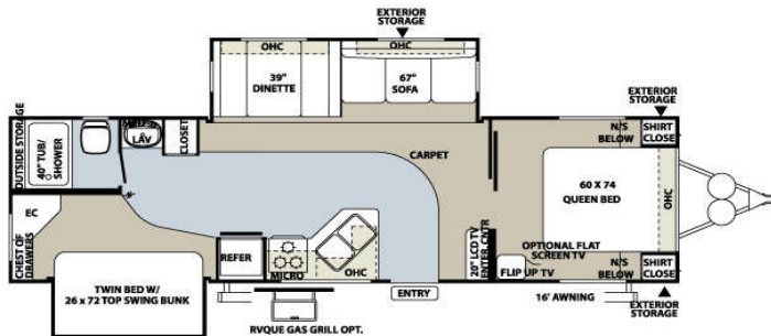
831BHSS 34'1" - 10,39m
