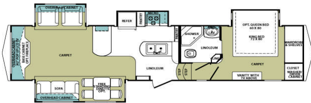
3515 RT 40' (12.2 m)
