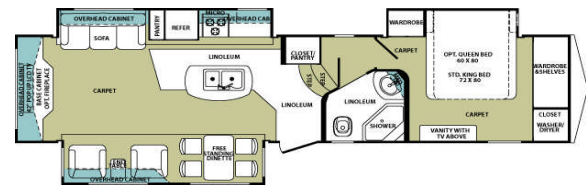
3625 RT 38' 6" (11.7 m)
