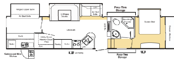
324FWBH 38'6" - 9,11m
