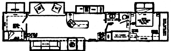
MARATHON 46 5th Wheel 2 BR 6 Slide
